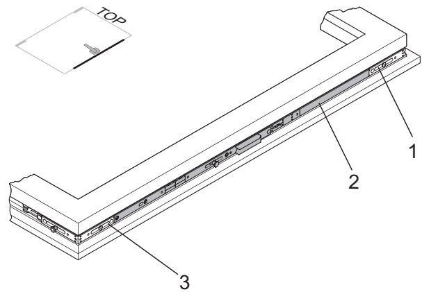
Засов GAM/GAK
