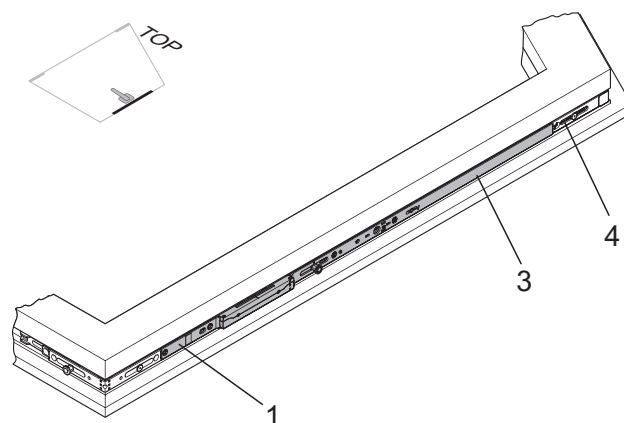
Засов GAM/GAK
